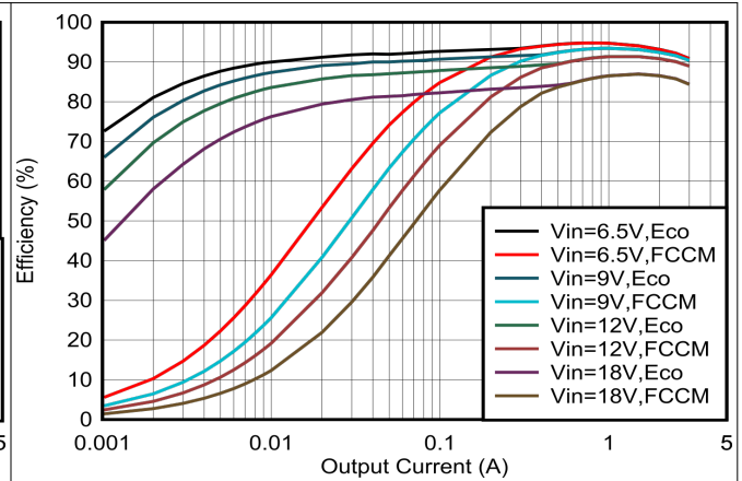
图 6-14. V_{OUT} = 3.3\text{-V} Efficiency, L = 2.2\text{ }\mu\text{H}
