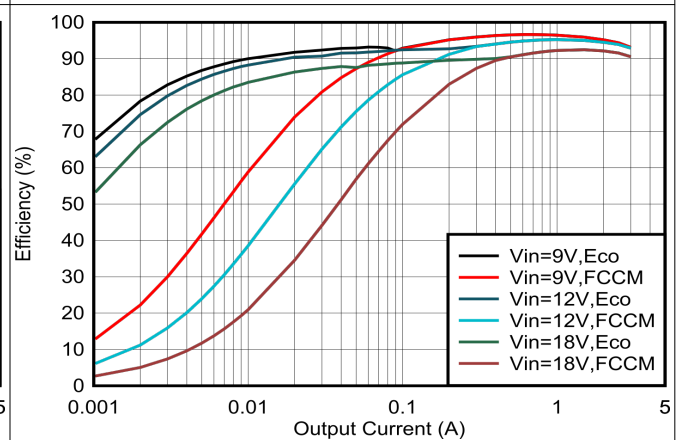
图 6-16. V_{OUT} = 7\text{-V} Efficiency, L = 3.3\text{ }\mu\text{H}
