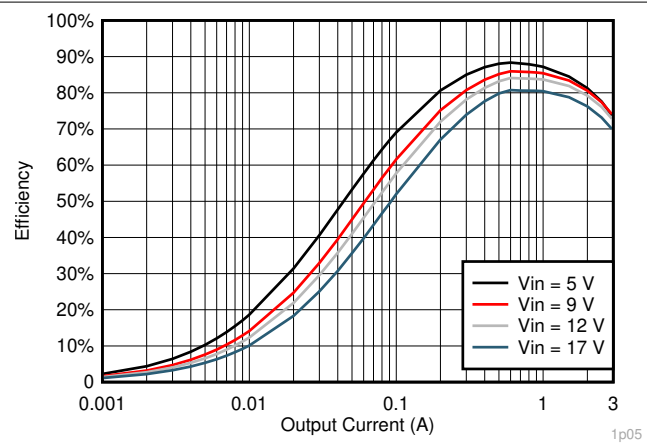
图 7-10. V_{OUT} = 1.05\text{-V} Efficiency, L = 1.5\ \mu\text{H}
