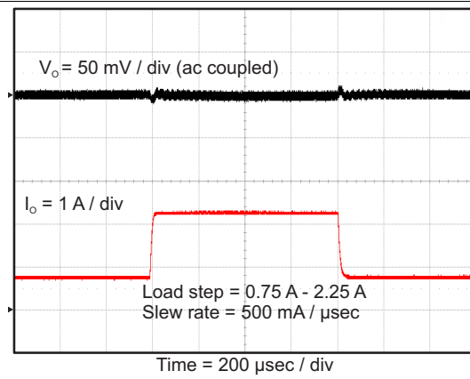
图 42. TPS563210A Transient Response
