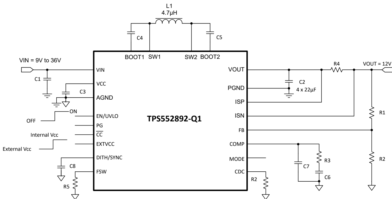
图 8-1. 12-V Power Supply With 9-V to 36-V Input Voltage
