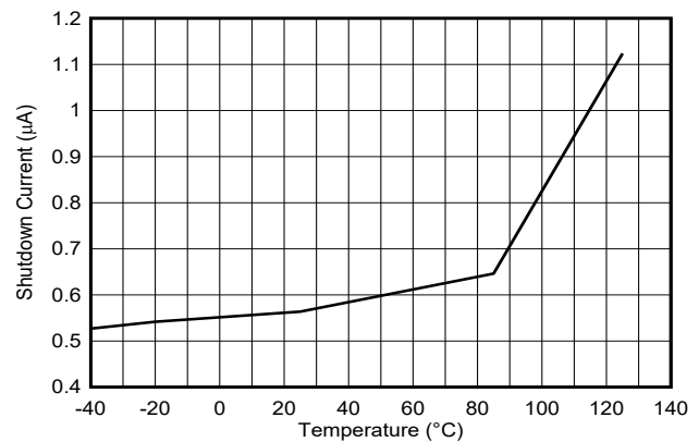
图 6-14. Shutdown Current vs Temperature
