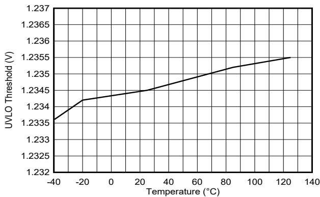
图 6-15. ENABLE/UVLO Rising Threshold vs Temperature
