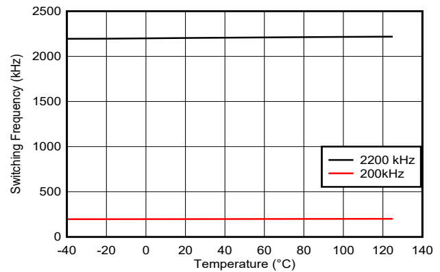
图 6-16. Switching Frequency vs Temperature
