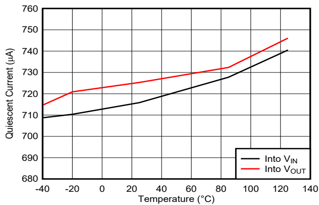
图 6-13. Quiescent Current vs Temperature
