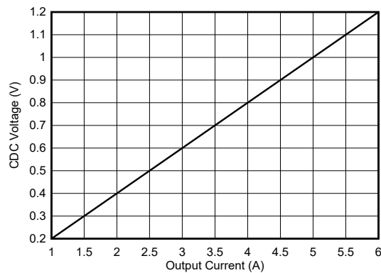
图 6-17. CDC Voltage vs Output Current with R_{SENSE} = 10\text{ m}\Omega
