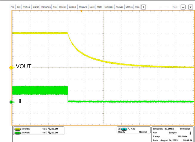
图 8-9. Shutdown Waveforms in V_{IN} = 16\text{ V} , V_{OUT} = 12\text{ V} , R_{LOAD} = 6\ \Omega , FPWM
