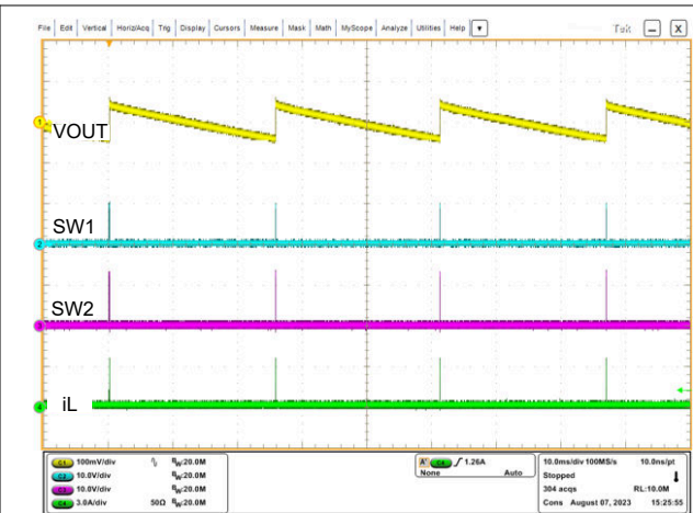
图 8-7. Switching Waveforms in V_{IN} = 9\text{ V} , V_{OUT} = 12\text{ V} , I_O = 0\text{ A} , PFM
