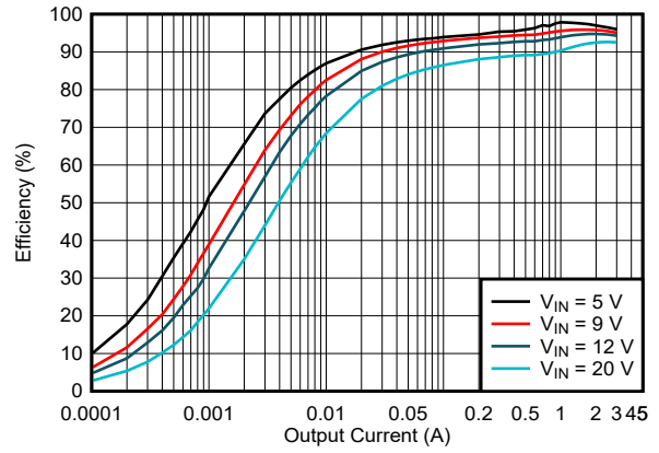
图 6-2. Efficiency vs Output Current, V_{OUT} = 5\text{ V} , f_{SW} = 400\text{ kHz} , PFM
