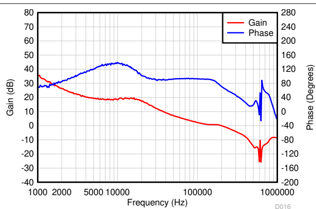
图 6-20. Frequency Response, 20 A Load
