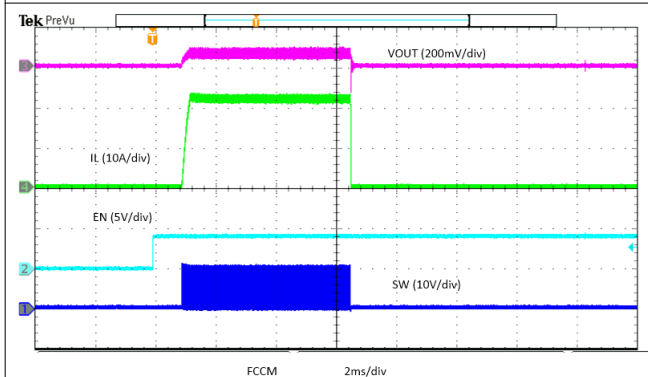
图 8-34. Enabled into Overcurrent
