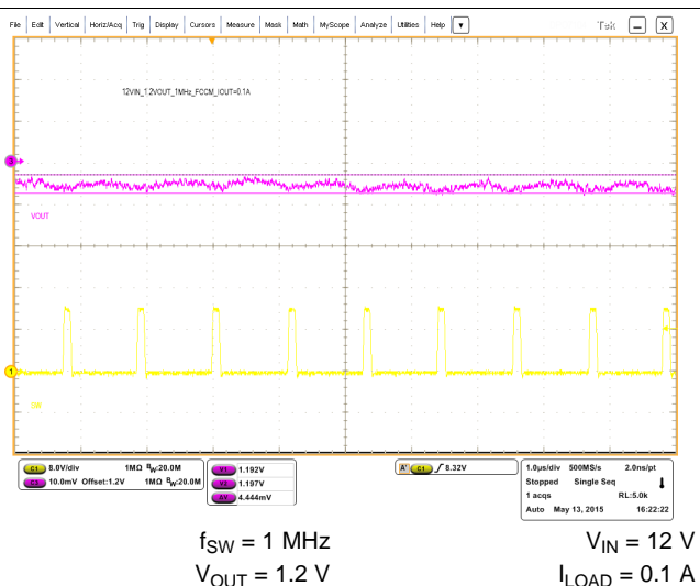
图 15. Steady-State Operation
