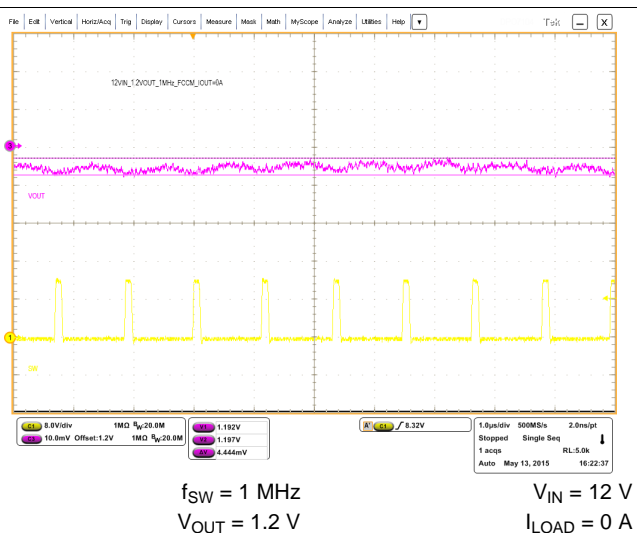
图 13. FCCM Steady-State Operation
