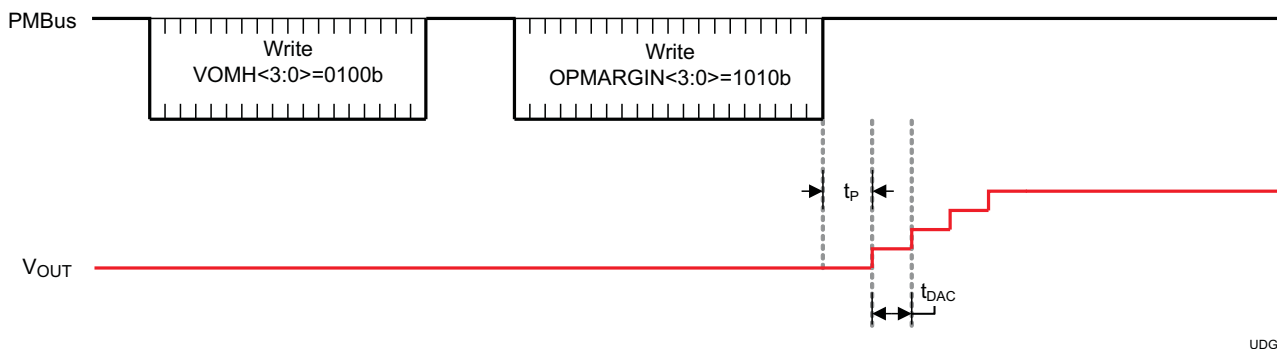
图 42. Setting the Margining Level First
