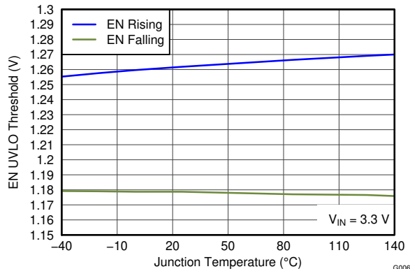
图 6-5. UVLO Threshold vs Temperature
