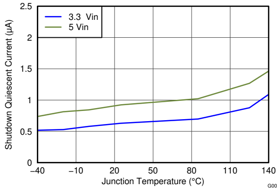
图 6-1. Shutdown Supply Current vs Temperature
