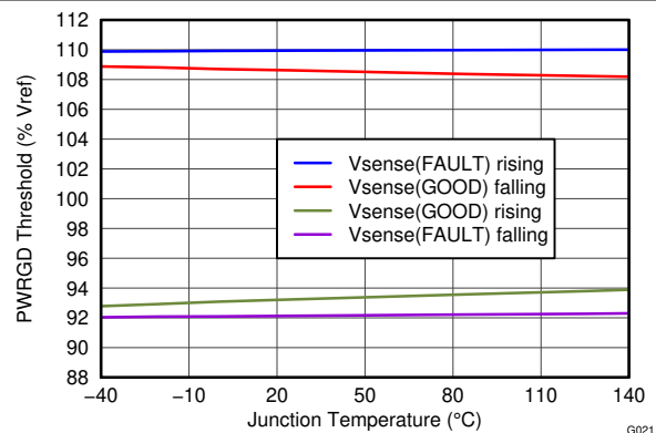
图 6-20. PWRGD Threshold vs Temperature
