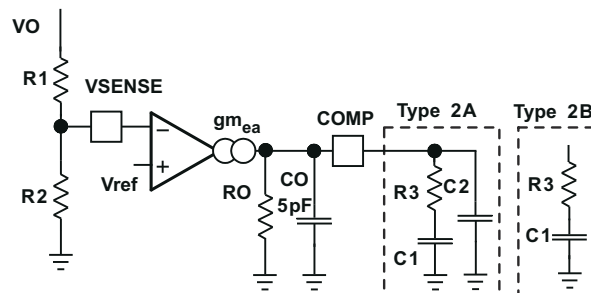
图 7-11. Types Of Frequency Compensation
