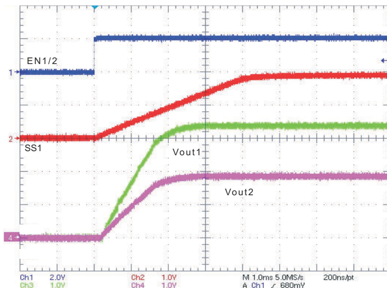
图 7-6. Ratio-Metric Start-Up With V_{OUT1} Leading V_{OUT2}
