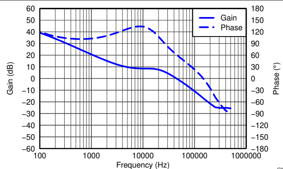
图 8-11. Closed Loop Response, VIN = 5 V, IOUT = 3.5 A
