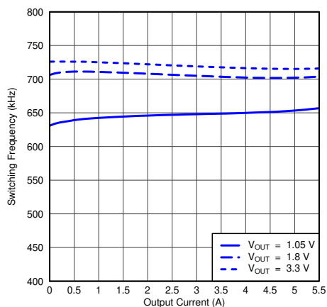
图 8-8. Switching Frequency vs Output Current
