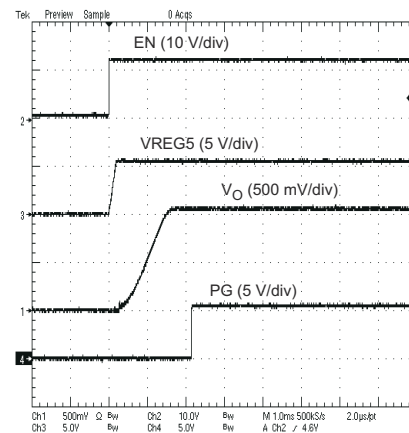
图 8-5. Start-Up Waveform
