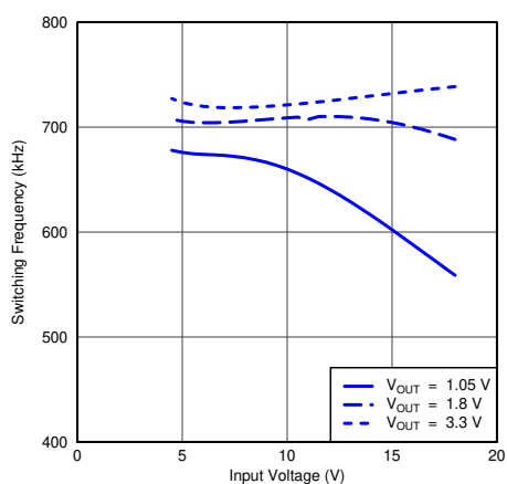
图 6-9. Switching Frequency vs Input Voltage ( I_O = 1\text{ A} )
