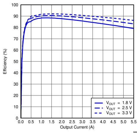
图 8-6. Efficiency vs Output Current
