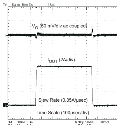
图 6-6. 1.05-V, 50-mA to 5.5-A Load Transient Response
