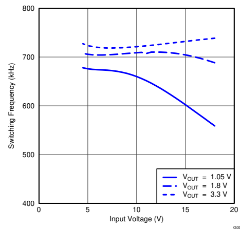
图 8-7. Switching Frequency vs Input Voltage ( I_O = 1 A)
