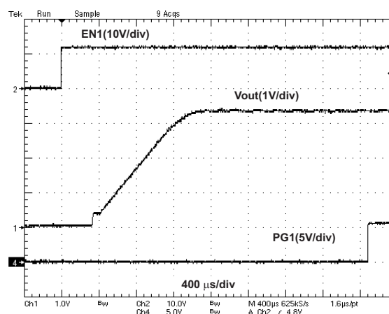
Figure 10. VO1=3.3V, PG1
