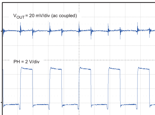
Figure 46. Output Ripple, I_{OUT} = 4 A
