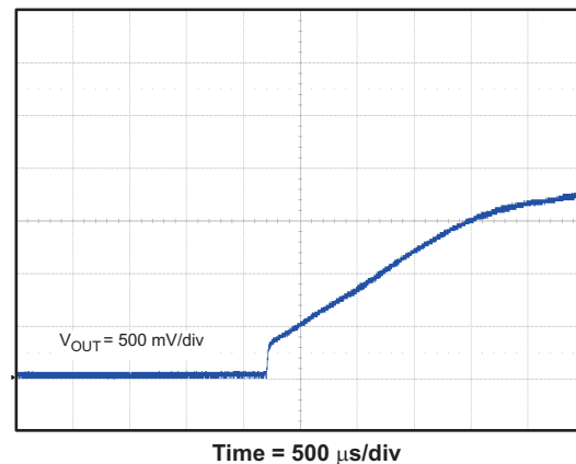
Figure 53. Start Up Characteristic
