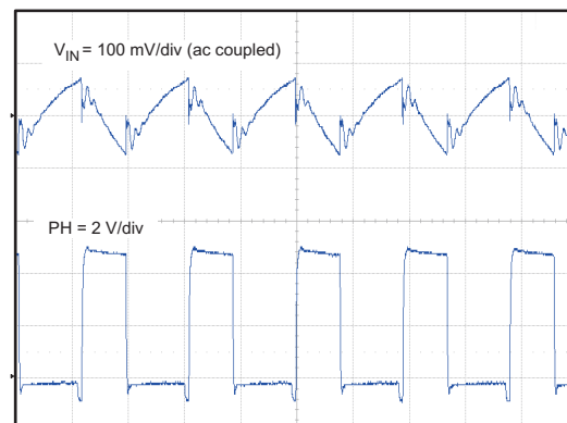
Figure 47. Input Ripple, I_{OUT} = 4 A
