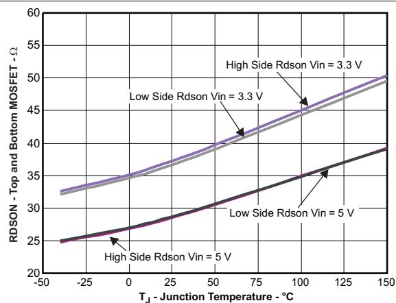
Figure 6. MOSFET Rdson vs Temperature
