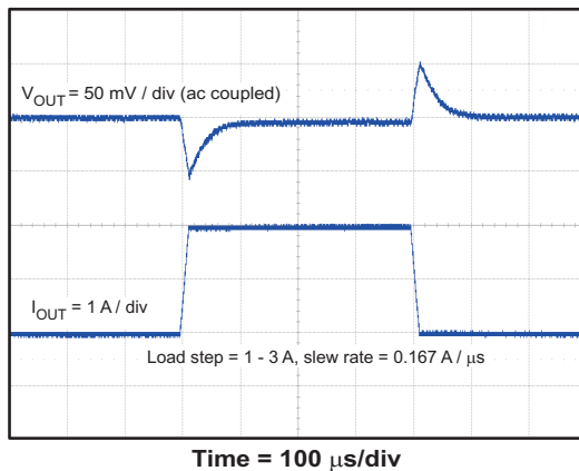
Figure 40. Transient Response, 2 A Step
