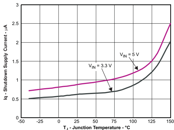
Figure 1. Shutdown Supply Current vs Temperature
