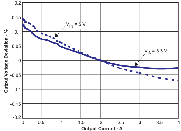
Figure 49. Output Voltage Regulation vs Load Current
