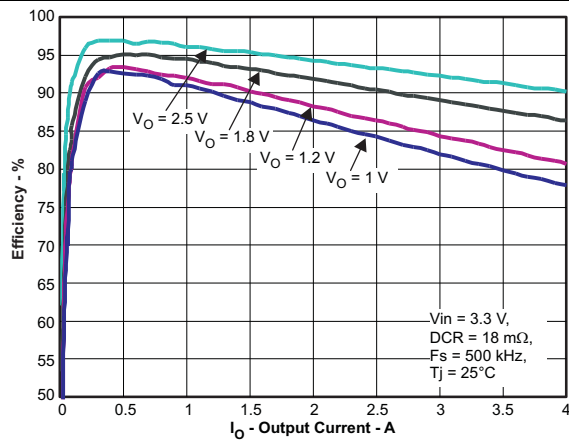
Figure 19. Efficiency vs Load Current
