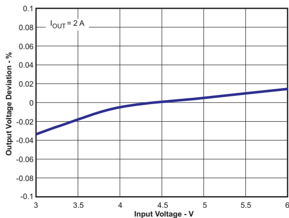
Figure 50. Output Voltage Regulation vs Input Voltage
