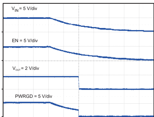
Figure 44. Power Down VOUT, VIN
