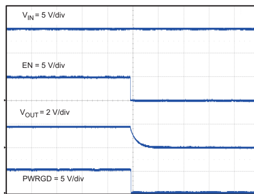
Figure 45. Power Down VOUT, EN
