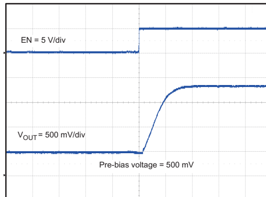
Figure 43. Power Up into Prebias Voltage
