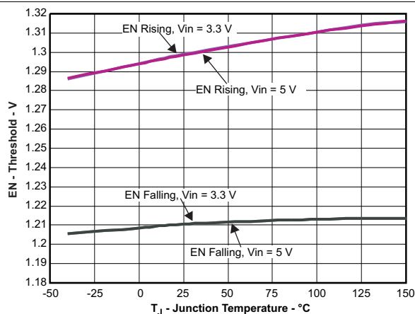
Figure 3. EN Pin Voltage vs Temperature
