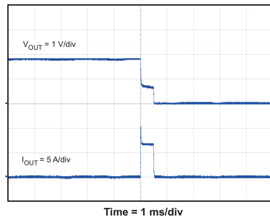
Figure 51. Hiccup Mode Current Limit
