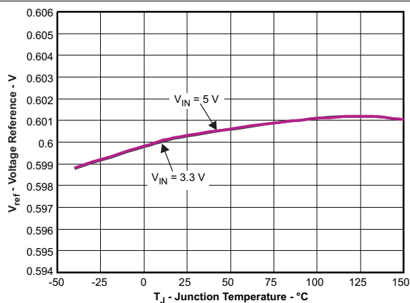
Figure 5. Voltage Reference vs Temperature
