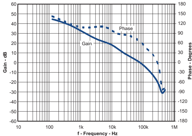
Figure 48. Closed Loop Response, V_{IN} = 5\text{ V} , I_{OUT} = 4\text{ A}
