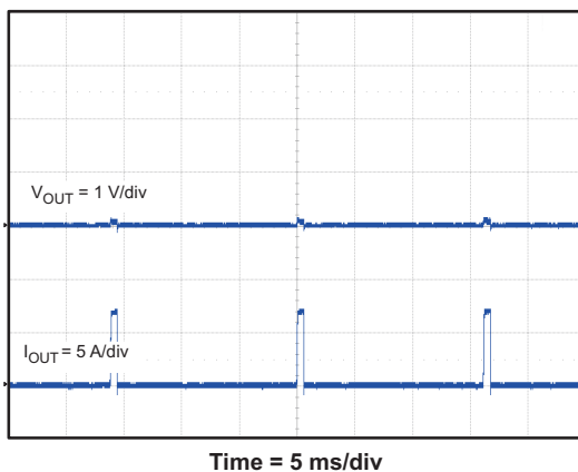
Figure 52. Hiccup Mode Current Limit
