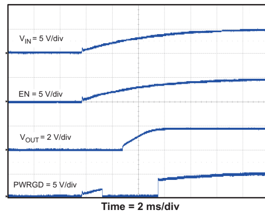
Figure 41. Power Up VOUT, VIN
