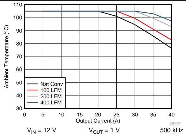
图 44. Safe Operating Area
