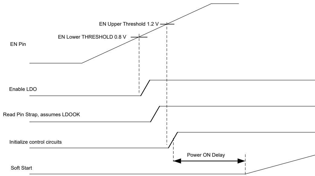
Figure 6-3. Internal Start-Up Sequence
