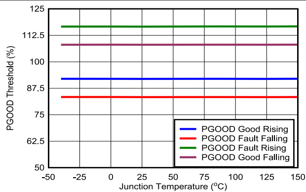
Figure 5-9. PG Threshold
