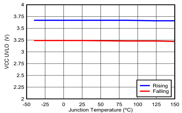
Figure 5-8. V_{CC} UVLO
