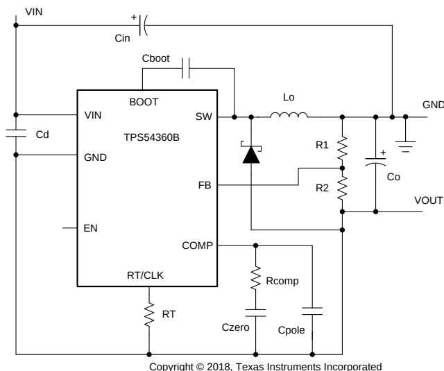
Figure 50. TPS54360B Inverting Power Supply
