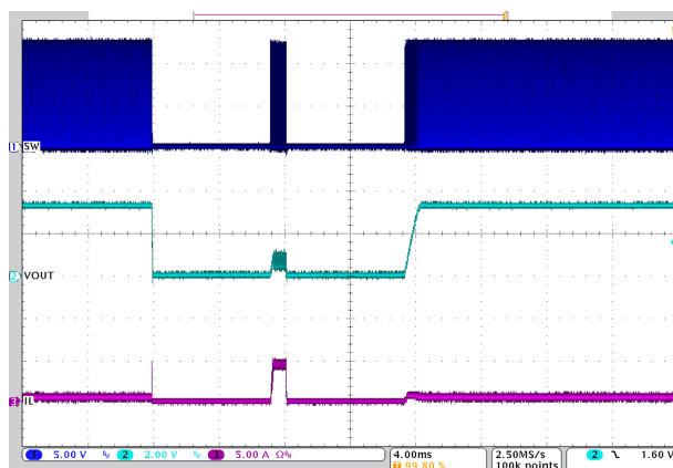
V_{IN} = 12\text{ V} 图 8-20. Overcurrent Protection - Hiccup and Recover
