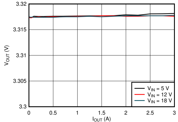
图 8-5. Load Regulation
