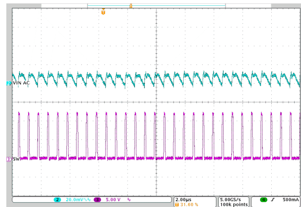
V_{IN} = 12\text{ V} I_{OUT} = 0\text{ A} 图 8-29. Input Ripple - No Load
