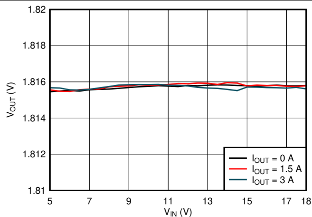
图 8-24. Line Regulation
