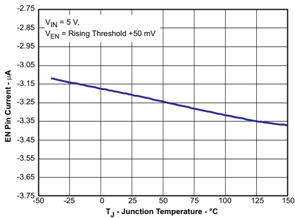
Figure 11. Pin Current vs Junction Temperature
