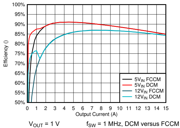
图 6-3. Efficiency vs Output Current
