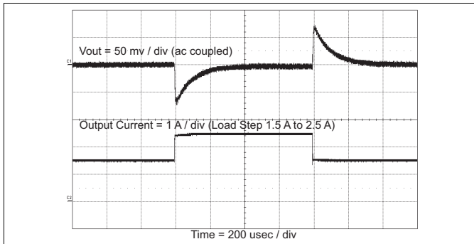
Figure 47. Load Transient
