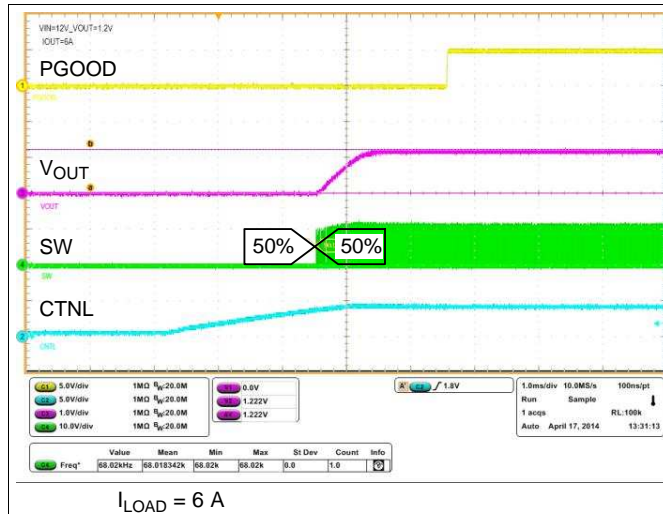
图 57. Start-Up Sequence
