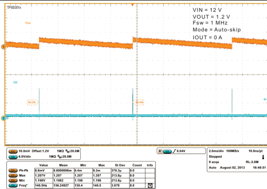
图 13. Auto-Skip Steady-State Operation
