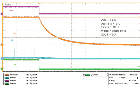
图 25. Shutdown Operation
