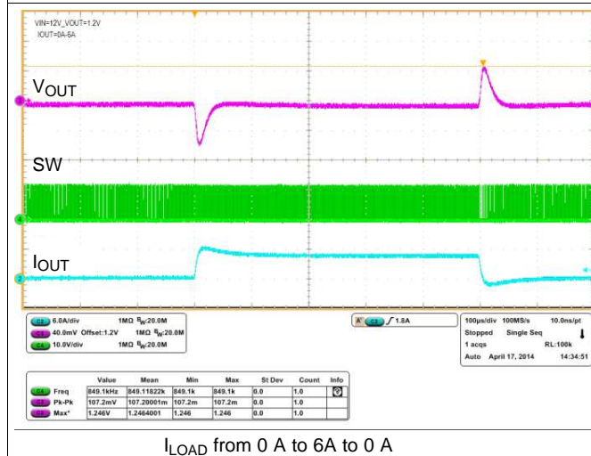
图 61. Full Cycle Load Transient
