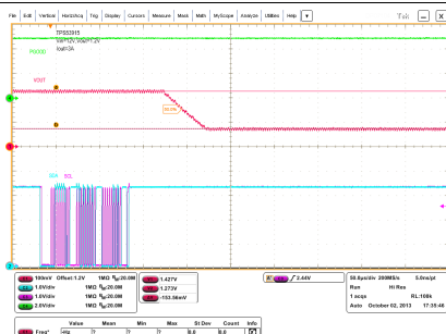
图 35. V OUT(adj) = 6%, V OH = 12% to 0%
