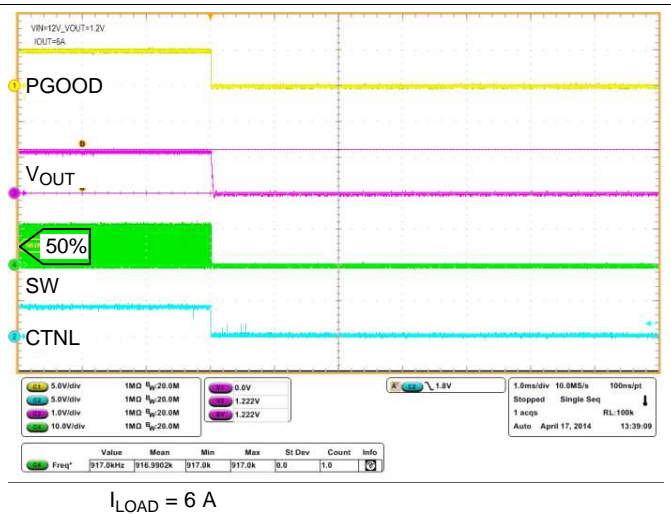
图 58. Shutdown Sequence
