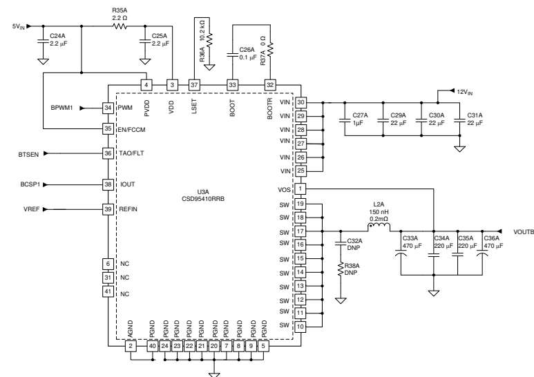
图 8-3. Powerstages Schematic (2/2)
