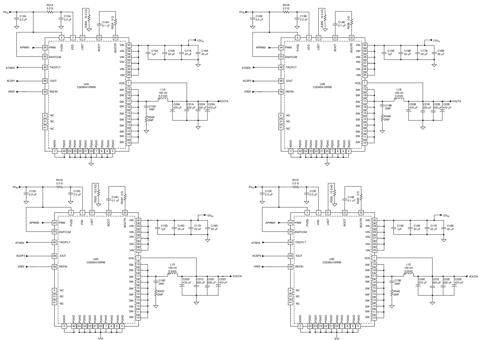
图 8-2. Powerstages Schematic (1/2)
