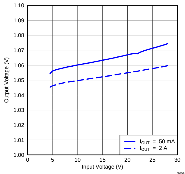
图 9. Line Regulation
