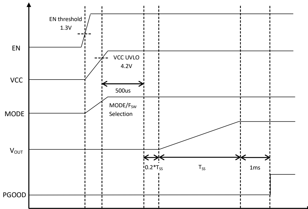
图 7-1. Power-Up Sequence
