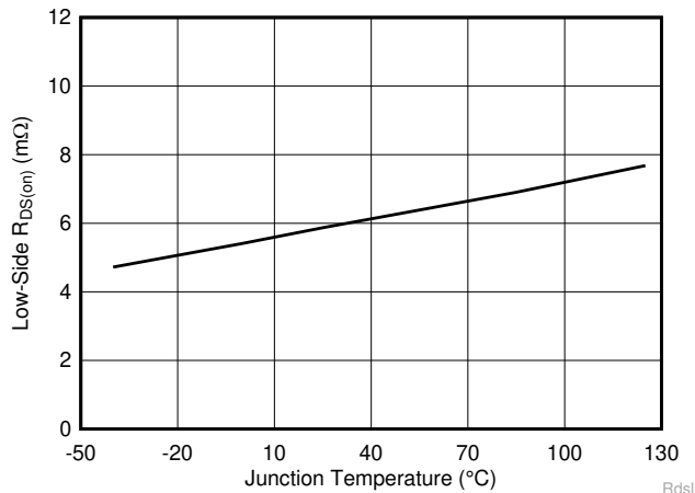
图 6-7. Low-Side R_{DS(on)} vs Junction Temperature
