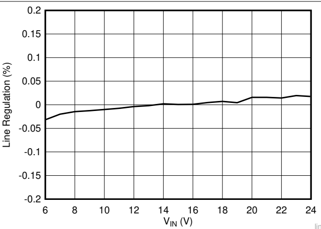
图 8-6. Line Regulation, I_{OUT} = 0.1\text{ A}
