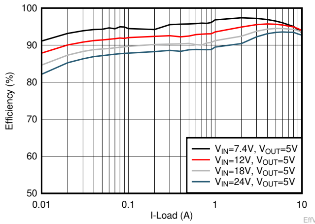
图 8-2. Efficiency Curve
