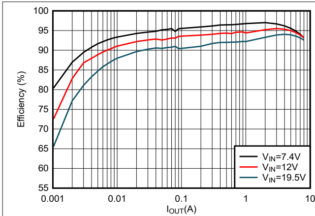
图 8-2. Efficiency, PSM Mode
