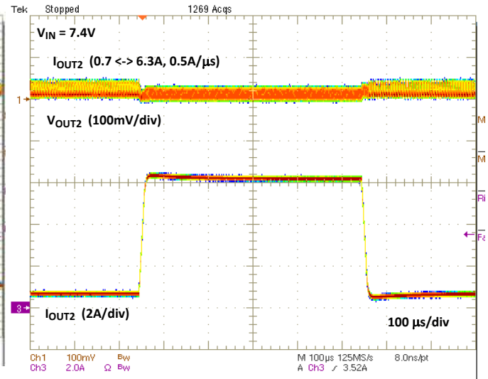
Figure 26. Load Transient
