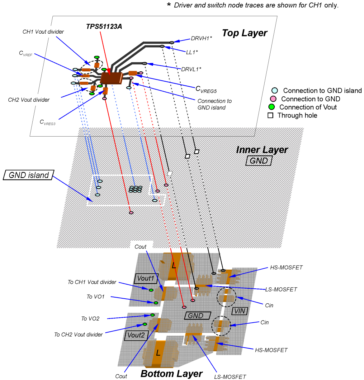
Figure 38. PCB Layout
