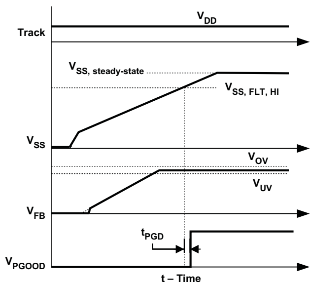
Figure 35. PGOOD Signal
