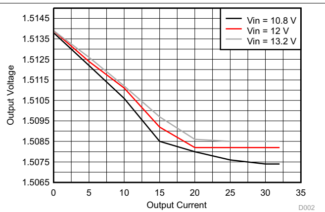
Figure 54. Load Regulation
