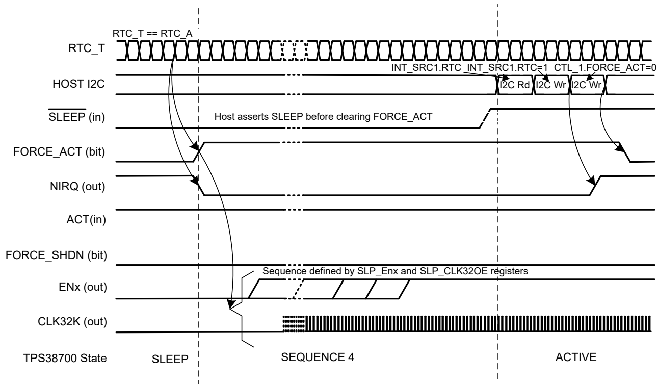
图 8-11. Sleep Exit RTC Triggered - Autonomous Sequencing
