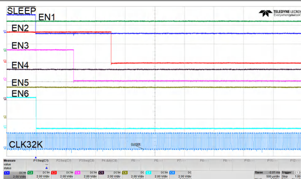
图 9-4. Sleep Entry Sequence
