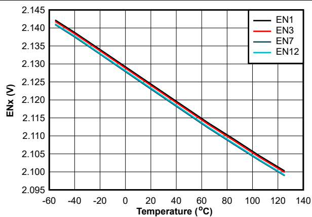
图 7-8. ENx Logic High Output Voltage vs. Temperature
