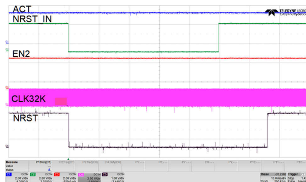
图 9-6. RESET Triggered by NRST_IN
