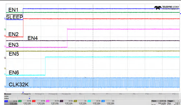
图 9-5. Sleep Exit Sequence
