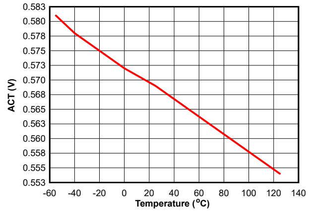
图 7-2. ACT Logic Low Threshold Voltage vs. Temperature
