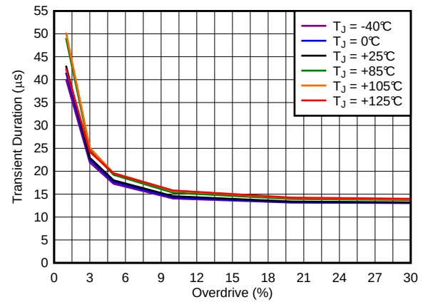
图 17. Minimum Transient Duration vs Overdrive (VDD = 5.5 V)
