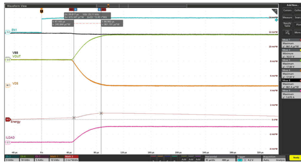
VBB = 13.5V IOUT1 = 5A TAMB = 25°C VEN = 0V 至 5V
