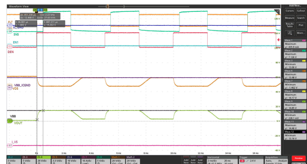
VBB = 13.5V VOUT = 开路负载 TAMB = 25°C DIAG_EN = PWM VEN1 = 0V SEL = 0 (200Hz)
