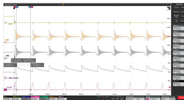
VBB = 13.5V ZOUT1 = 1uH + 100mΩ TAMB = 125°C VEN1 = 5V
