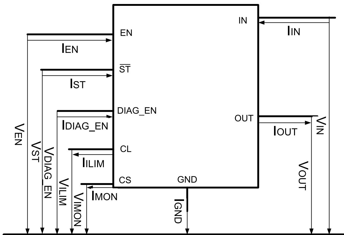
Figure 1. Pin Current and Voltage Conventions
