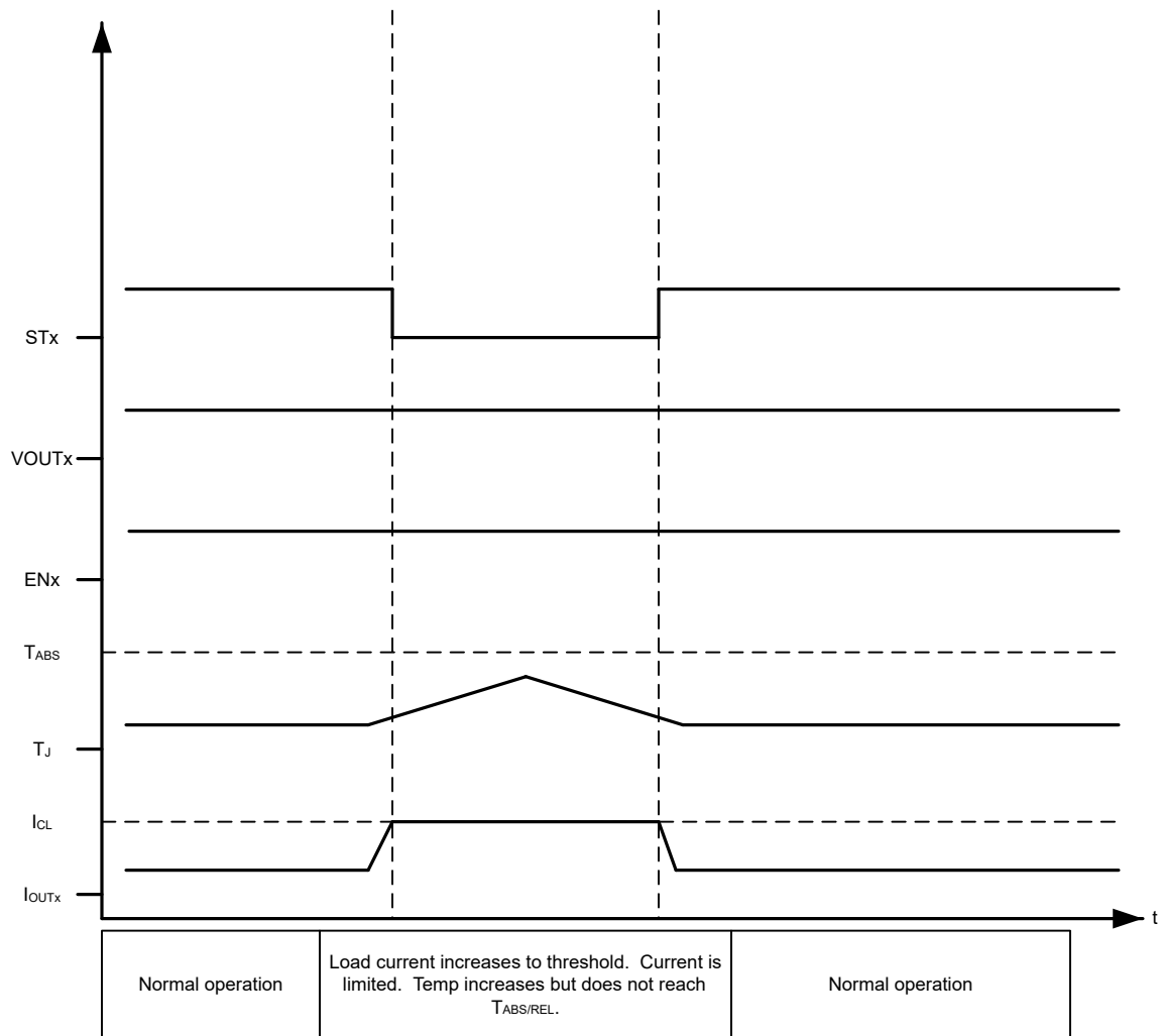
图 8-20. Overcurrent Behavior
