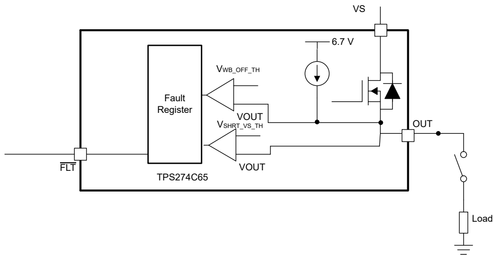
图 8-36. Open Load Detection Circuit
