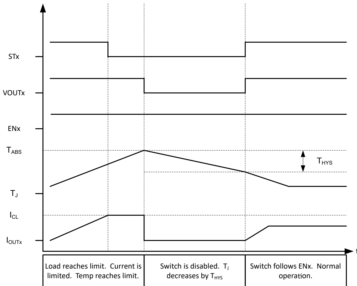
图 8-33. Current Limit - \text{AUTO\_RETRY\_DIS} = 0
