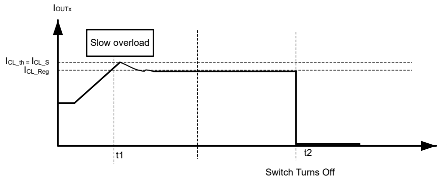
图 8-19. Overload Response
