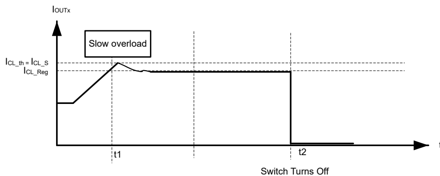
图 8-19. Overload Response
