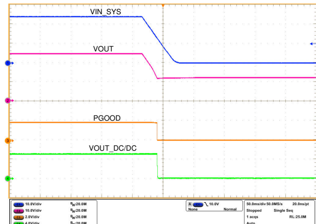
图 9-8. Power-Down Response
