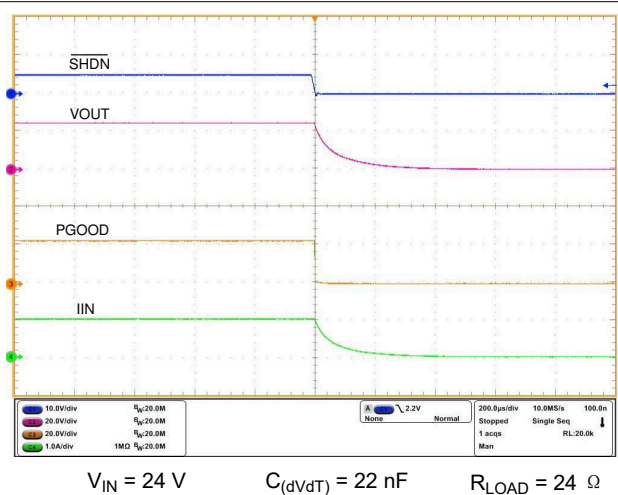
图 8-23. Turn-off Control with \overline{\text{SHDN}}
