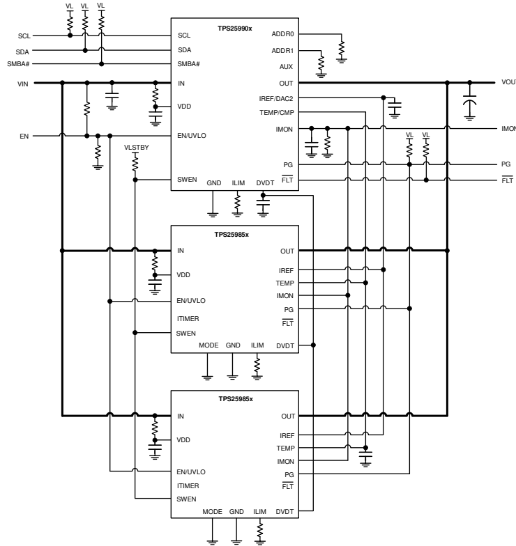
图 9-2. TPS25990 Connected in Parallel with TPS25985x For Higher Current Support With PMBus®
