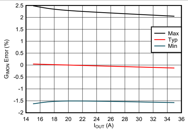
图 7-12. IMON Gain Accuracy Across Process, Voltage and Temperature Corners
