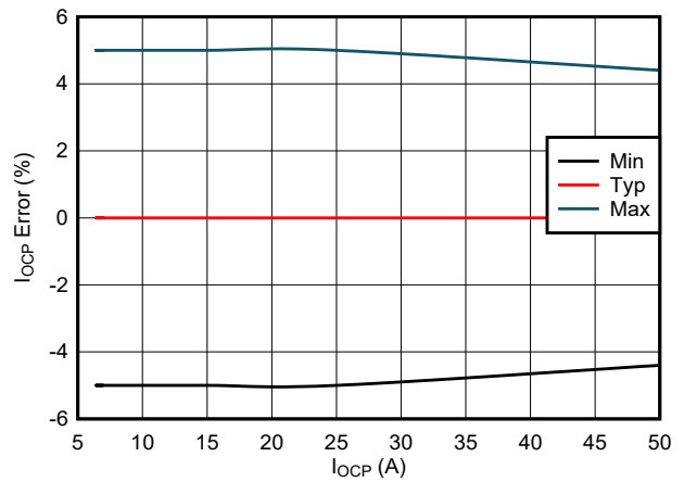
图 7-14. Steady-state Overcurrent Protection Threshold (Circuit-Breaker) Accuracy
