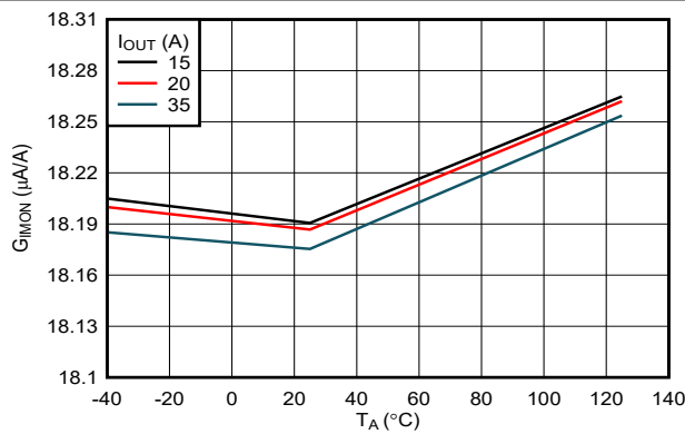
图 7-11. IMON Gain Across Load and Temperature
