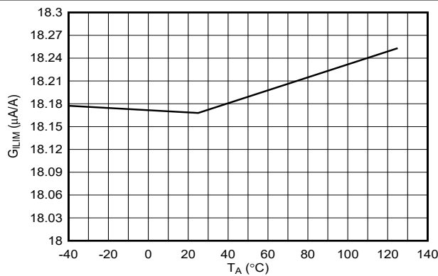
图 7-15. ILIM Gain Across Load and Temperature
