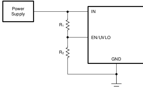
图 8-2. Adjustable Undervoltage Protection
