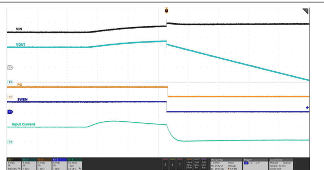
图 7-44. Input Undervoltage Protection
