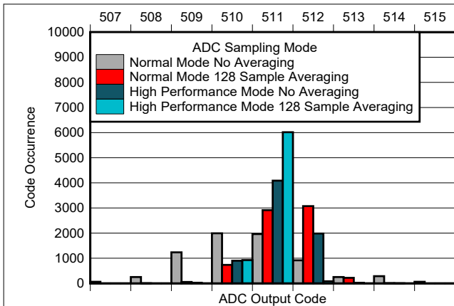
图 7-25. ADC Histogram (Mid-scale Analog Input)
