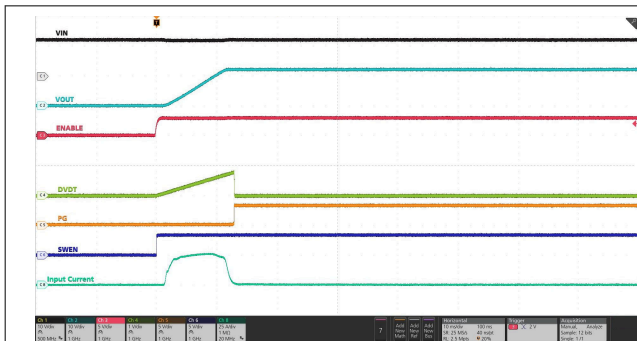
IN supply held steady at 12 V, EN toggled from low to high. C_{OUT} = 18\text{ mF} , C_{dVdt} = 33\text{ nF} , Default PG delay setting (DEVICE_CONFIG[15] = 0b)
