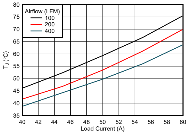
图 7-33. Junction Temperature vs Load Current (With Air-Flow)
