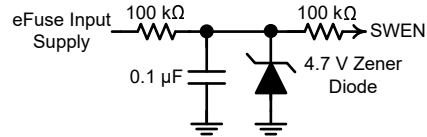
图 9-16. Zener Regulator Used as Pullup Supply for SWEN
