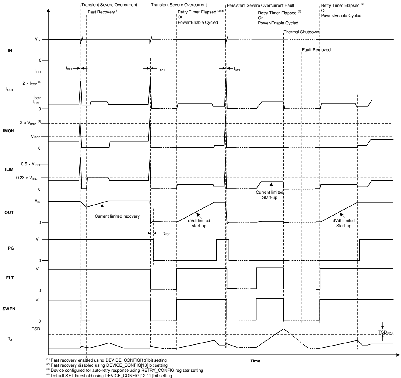
图 8-5. Short-Circuit Response
