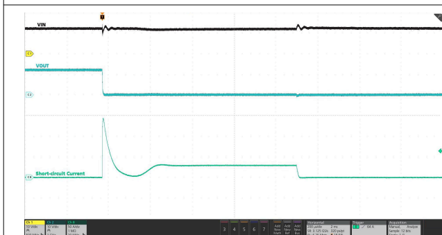
图 7-57. Short-Circuit Protection During Steady-state
