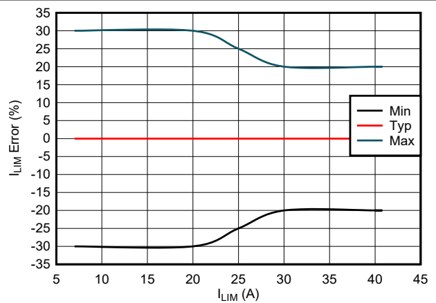
图 7-16. Startup Overcurrent Protection Threshold (Current Limit) Accuracy
