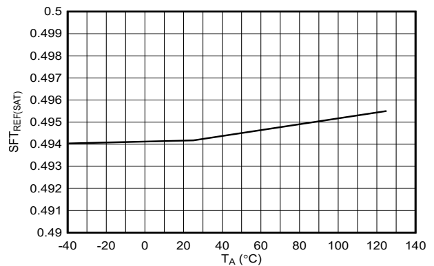
图 7-18. Scalable Fast-trip Threshold Ratio Across Temperature (Startup)
