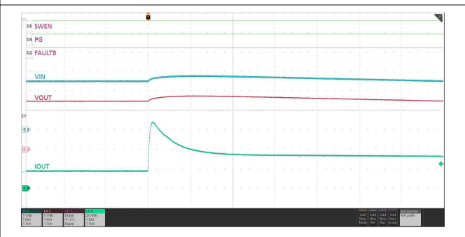
图 7-58. Short-Circuit Protection During Steady-state
