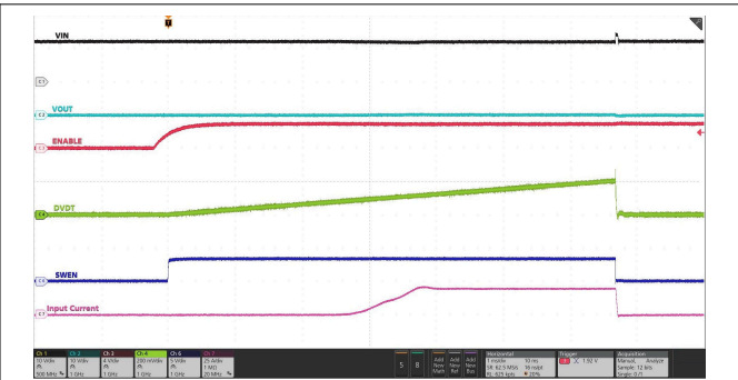
图 7-56. Power Up into Short-Circuit Protection
