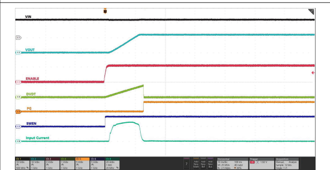
IN supply held steady at 12 V, EN pin toggled from low to high. C_{OUT} = 18\text{ mF} , C_{dVdt} = 33\text{ nF}
