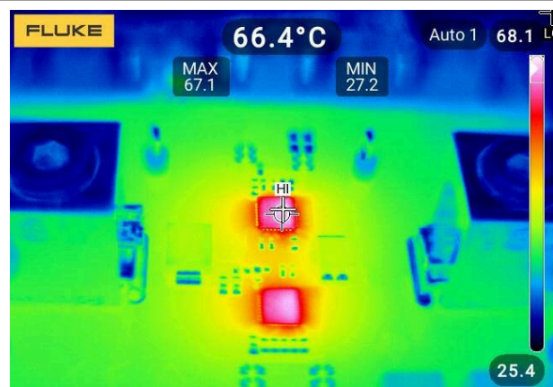
图 9-14. One (1) TPS25990 eFuse and one (1) TPS25985x eFuse in Parallel: Temperature Rise with 110-A DC Current at Room Temperature (No Air-Flow)
