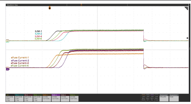
图 9-8. Power Up into Short (Current distribution among six devices in parallel): V_{IN} = 12 V, EN/UVLO Stepped Up From 0 V to 3 V, V_{IREF} = 1 V, R_{ILIM(TPS25990)} = 422 \Omega , R_{ILIM(TPS25985)} = 316 \Omega , and OUT Shorted to GND
