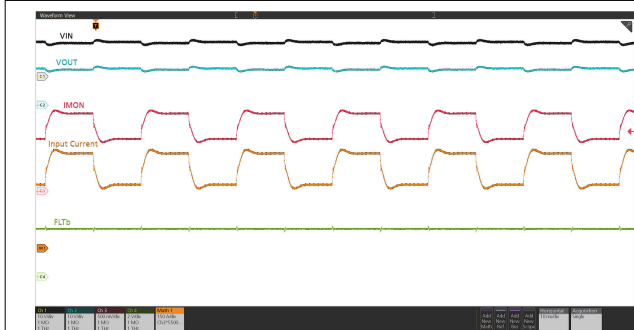
图 9-9. Transient Overload: V_{IN} = 12 V, t_{OC\_TIMER} = 10 ms, C_{LOAD} = 50 mF, R_{IMON} = 150 \Omega , V_{IREF} = 1 V, and Load Current Stepped from 333 A to 500 A then 333 A within 8.5 ms
