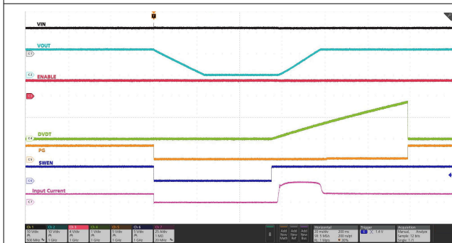
IN supply held steady at 12 V, EN pin held high, PMBus POWER_CYCLE Command. C_{OUT} = 18\text{ mF} , C_{dVdt} = 33\text{ nF} , Default delay setting (RETRY_CONFIG[2:0] = 000b)
