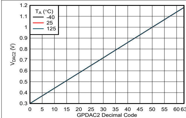
图 7-27. General Purpose DAC2 Transfer Function
