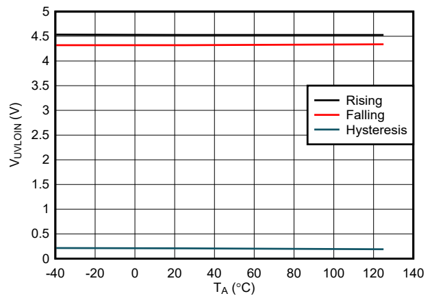
图 7-4. VIN Undervoltage Thresholds Across Temperature (VIN_UV_FLT = 0x38)
