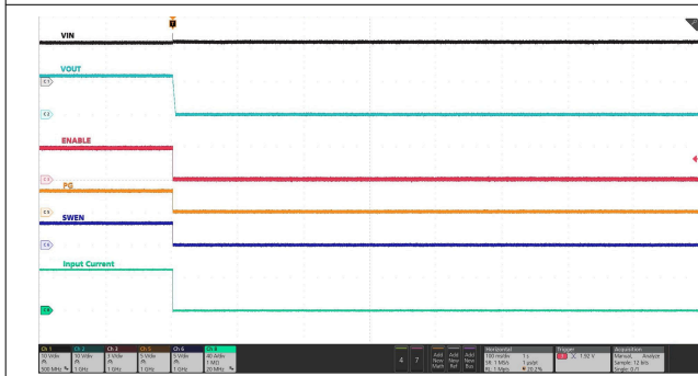
IN supply held steady at 12 V, EN pin toggled from high to low. C_{OUT} = 18\text{ mF} , C_{dVdt} = 33\text{ nF} , I_{LOAD} = 50\text{ A}
