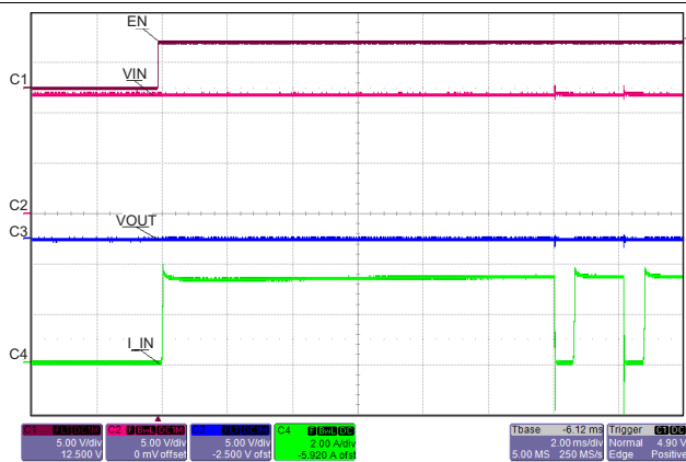
Figure 27. Short Circuit (Zoom): Fast-Trip Comparator
