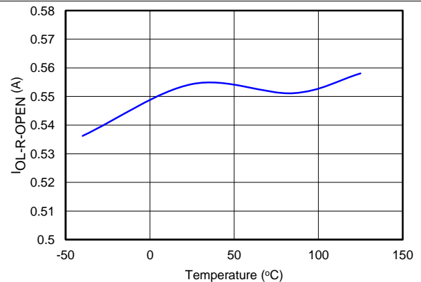
Figure 22. I_{OL} , I_{SC} vs Temperature
