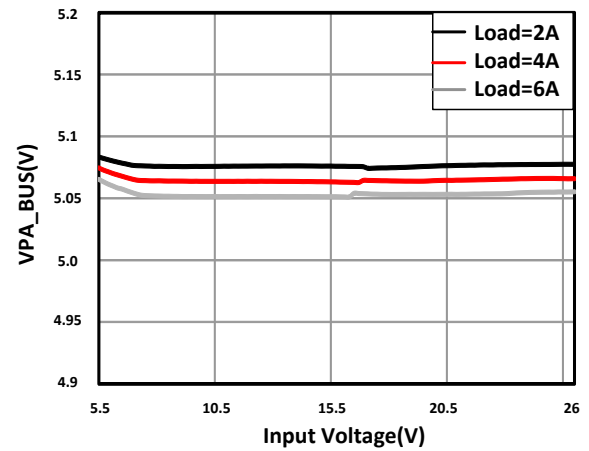
图 11-12. Dropout Characteristic
