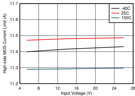
图 8-7. High-side Current Limit vs Input Voltage
