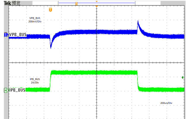
图 11-10. Load Transient With Cable Compensation
