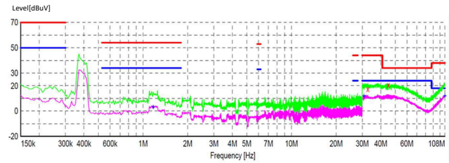
图 11-3. 400-kHz EMI Results (Without CM Filter)
