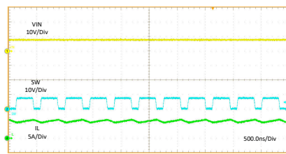
图 10-5. Switching Frequency When R_{FREQ} = 8.45 \text{ k}\Omega
