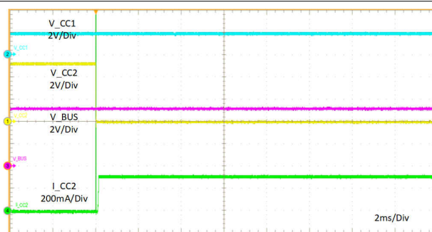
图 11-23. Short Circuit Recovery
