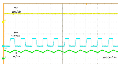
图 10-6. Switching Frequency When R_{FREQ} = 8.45 \text{ k}\Omega
