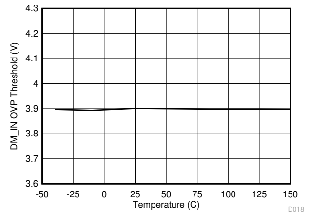
图 8-22. DM_IN Overvoltage Protection Threshold vs Junction Temperature
