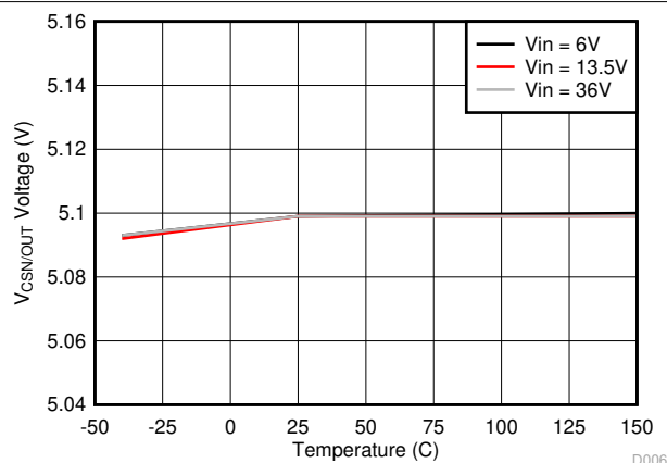
图 8-7. V_{CSN/OUT} Voltage vs Junction Temperature
