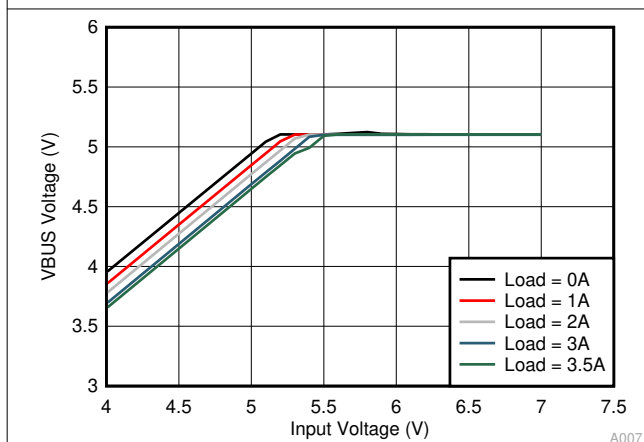
图 11-12. Dropout Characteristic
