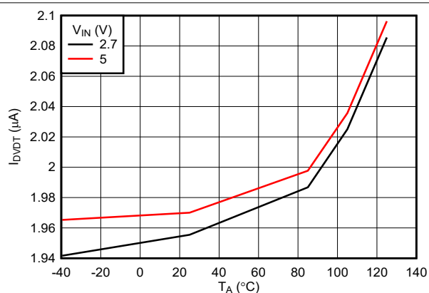
图 7-27. DVDIT Charging Current vs Temperature
