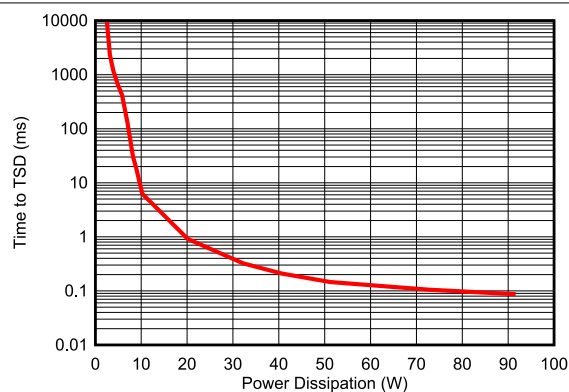
图 7-30. Time to Thermal Shut-Down During Inrush State
