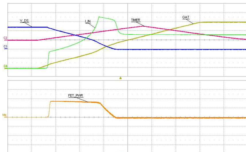
I_IN: Input Current, 2 A/div GAT: Voltage on GATE Pin, 5 V/div V_DS: Drain-to-Source Voltage of M1, 5 V/div TIMER: Voltage on TIMER Pin, 500 mV/div FET_PWR: Power on M1 (product of V_{DS} and I_{IN} ), 19 W/div Time: 10 ms/div
