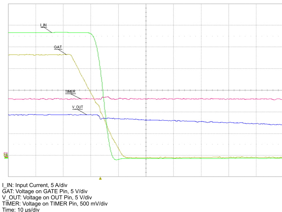
Figure 27. Current Limit During Output-Load Short-Circuit Condition (Onset)
