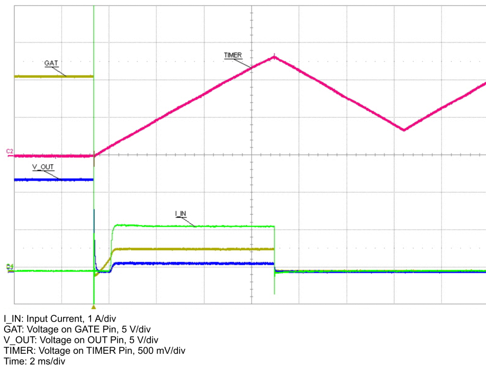
Figure 26. Current Limit During Output Load Short-Circuit Condition (Overview)
