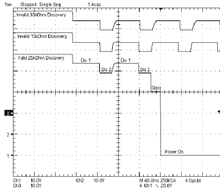
图 8-4. Invalid (33 kΩ and 15 kΩ) and Valid Discovery (25 kΩ)
