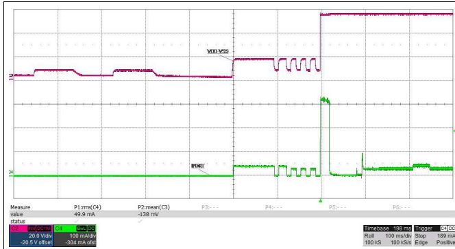
Figure 24. 启动
