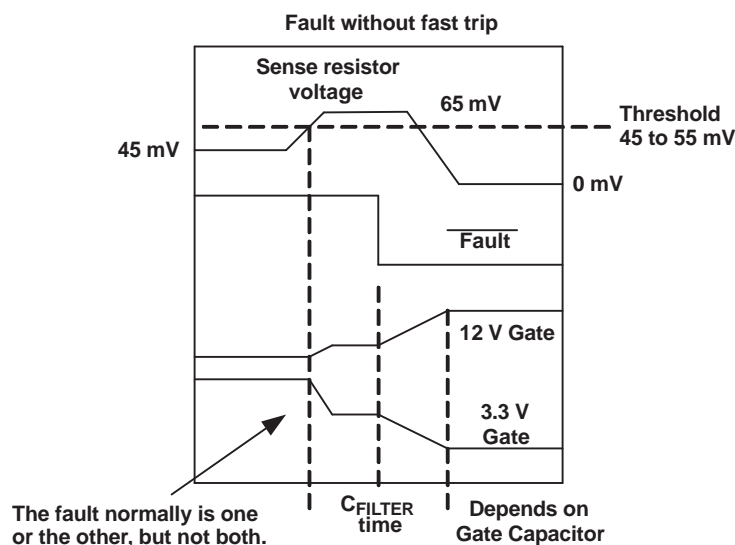
Figure 2. Fault Without Fast Trip
