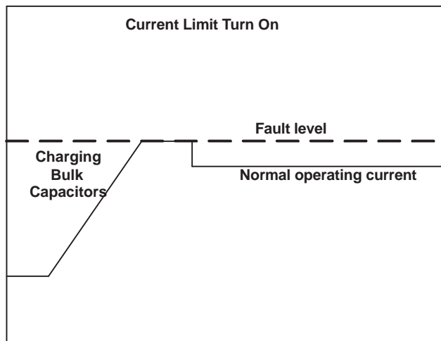
Figure 3. Hot Plug Current Limit Turn ON
