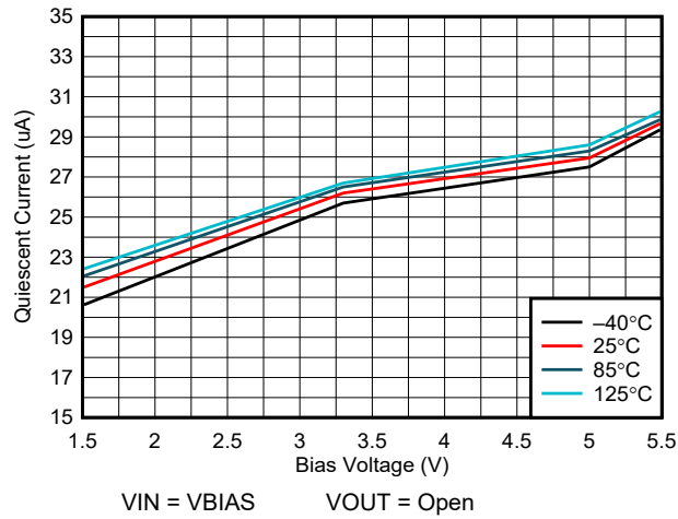
图 7-1. Quiescent Current vs Bias Voltage
