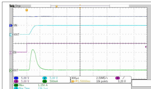
图 10-2. Inrush Current for C_L = 47 \text{ } \mu\text{F} with C_T = 0 \text{ pF}
