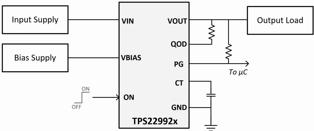
图 10-1. TPS22992x Typical Application
