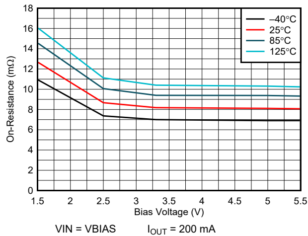
图 7-3. ON-Resistance vs Bias Voltage
