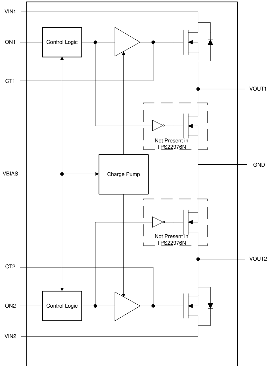
图 8-1. TPS22976 Functional Block Diagram
