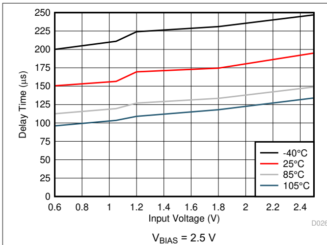
图 6-39. Delay Time vs Input Voltage
