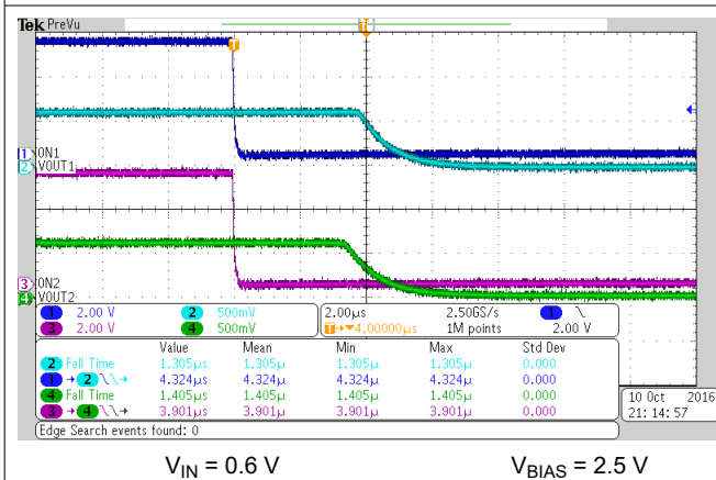
图 6-35. Turnoff Response Time
