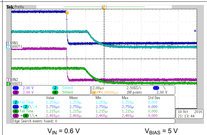
图 6-36. Turnoff Response Time
