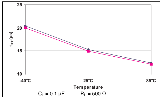
Figure 7. t_{OFF} vs Temperature ( V_{IN} = 1.8 V )
