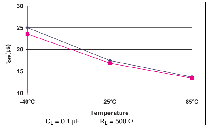
Figure 8. t_{OFF} vs Temperature ( V_{IN} = 3.6 V )
