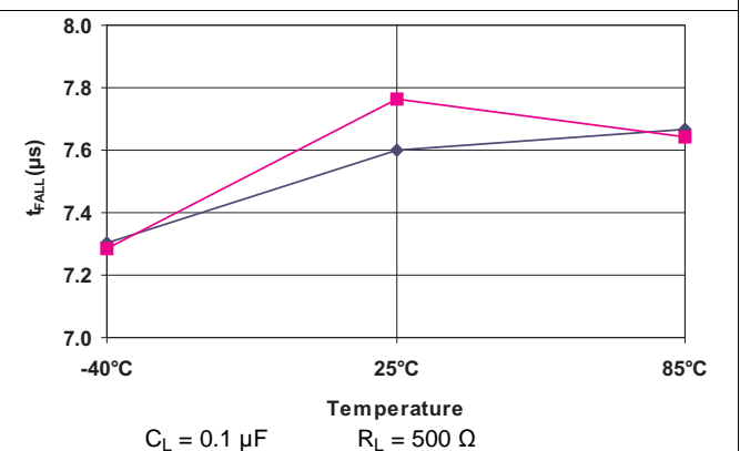
Figure 12. t_{FALL} vs Temperature ( V_{IN} = 3.6 V )
