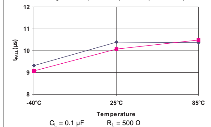
Figure 11. t_{FALL} vs Temperature ( V_{IN} = 1.8 V )
