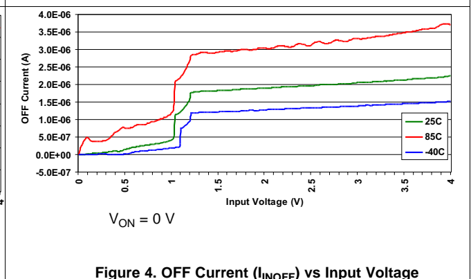
Figure 4. OFF Current ( I_{INOFF} ) vs Input Voltage
