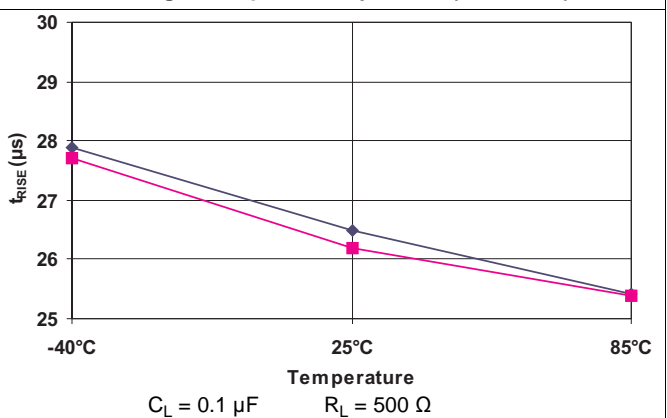
Figure 10. t_{RISE} vs Temperature ( V_{IN} = 3.6 V )
